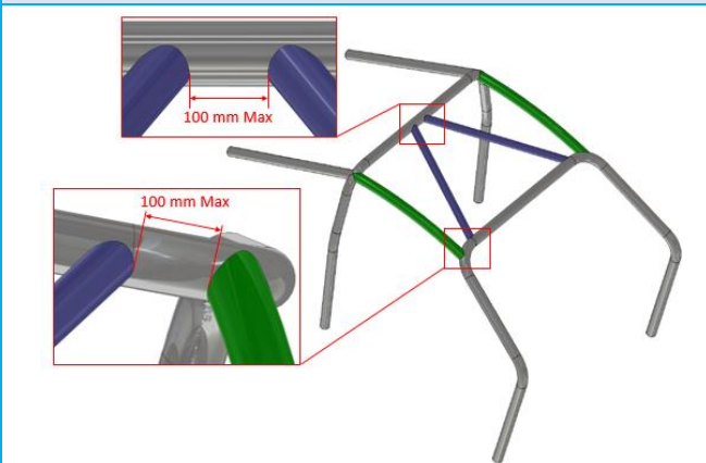
Dessin/Drawing SC-10a
