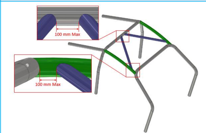
Dessin/Drawing SC-10b
