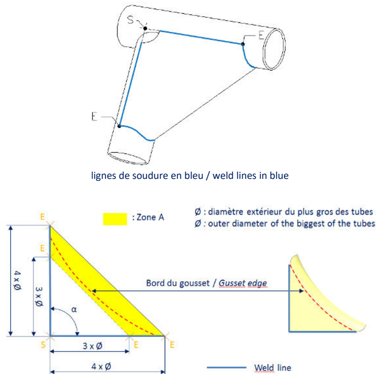
Dessin/Drawing SC-GU-1
