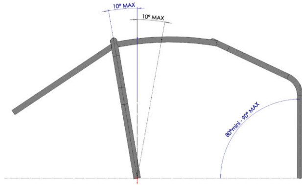
Dessin/Drawing SC-5
