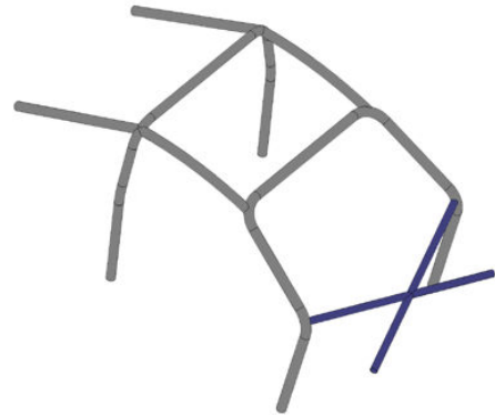
Dessin/Drawing SC-13b
